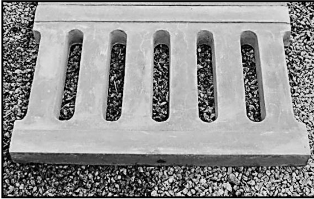
CONCRETE DRAIN COVER (600 X 390 X 50thk) CSL-CDC001
